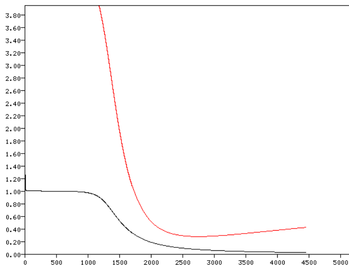
Figure 4: Error rate during training for a four node neural network trying to learn the XOR function.
