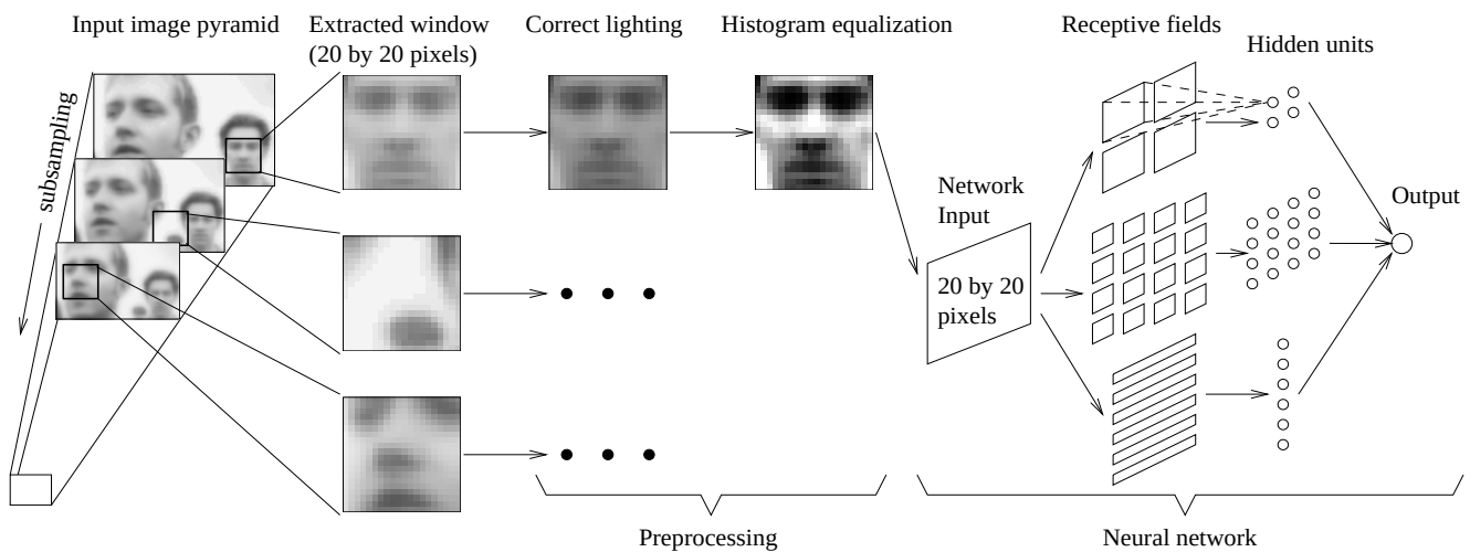
Figure 1: The basic algorithm used for face detection.
